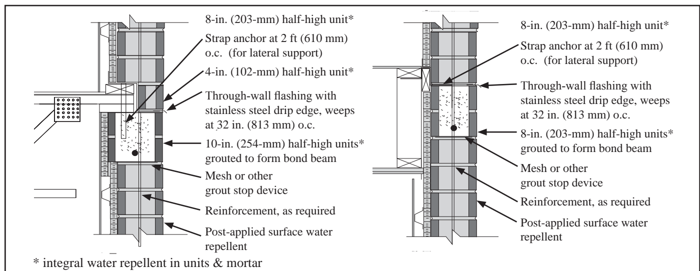
Figure 2—Exterior Loadbearing Wall With Wood Truss Floor (ref. 19)
