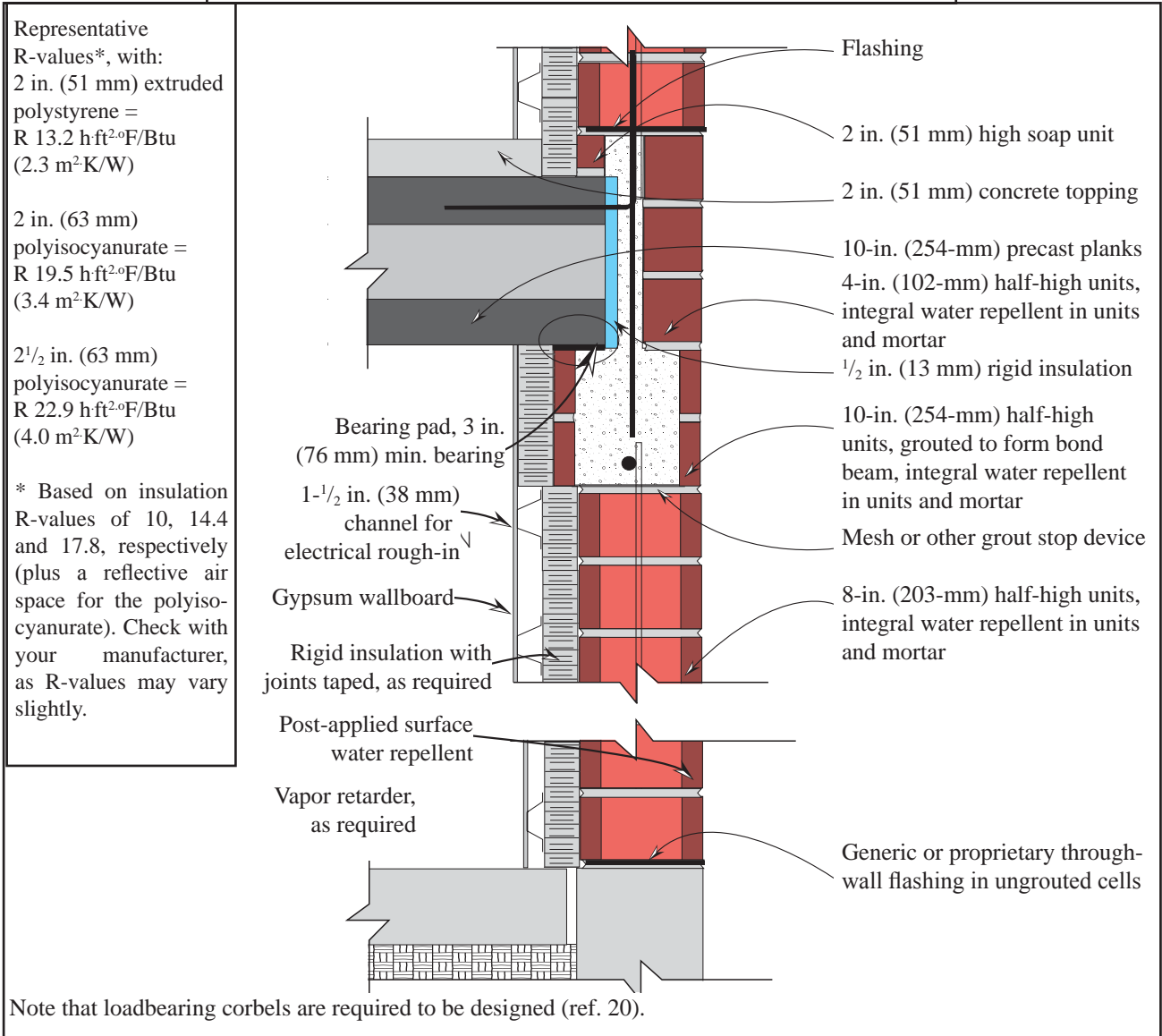
Figure 3—Exterior Wall With Precast Hollow Core Plank Floor (ref. 19)
