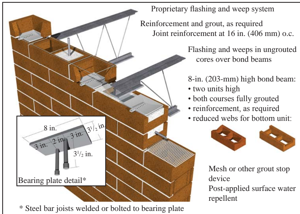
Figure 1—Bearing Detail on Single Wythe Wall (ref. 19)
